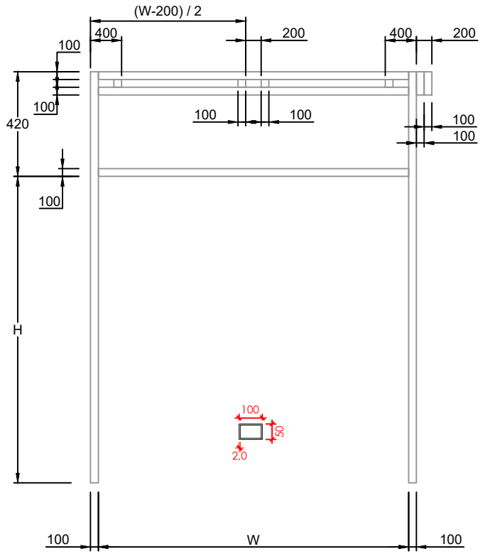
STANDART YATAKLAMALI (MOTOR SAĞDA) STANDARD LIFT (AUTOMATION ON RIGHT)
