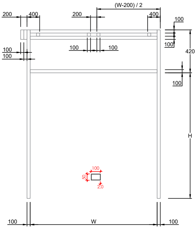
STANDART YATAKLAMALI (MOTOR SOLDA) STANDARD LIFT (AUTOMATION ON LEFT)
